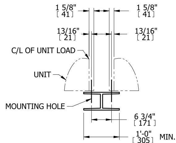
CENTER ARRANGEMENT
