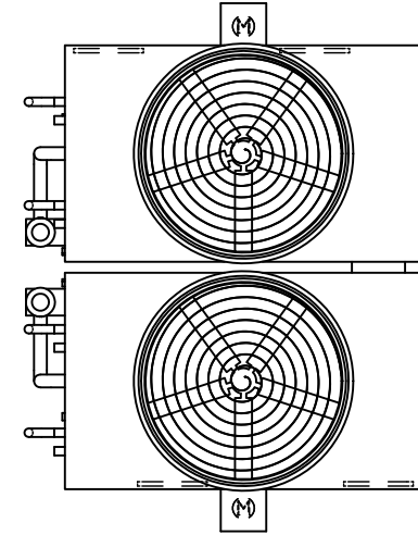
FACE 2 PLAN VIEW
