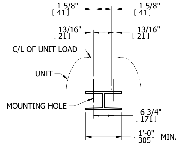
CENTER ARRANGEMENT
