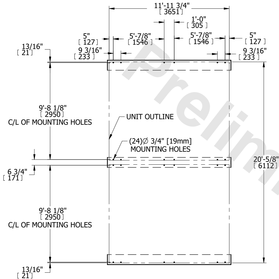
PLAN VIEW
