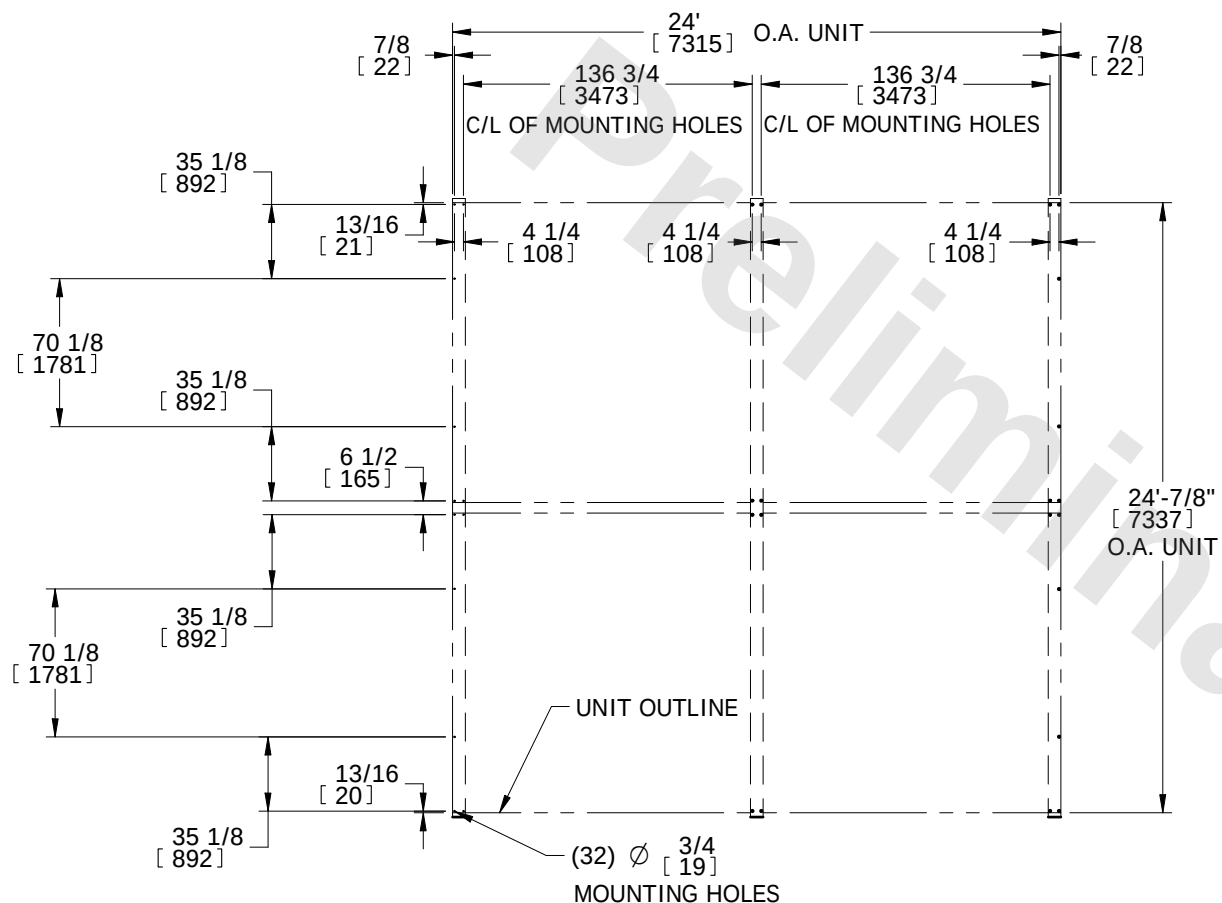
PLAN VIEW
