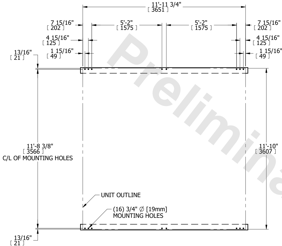
PLAN VIEW
