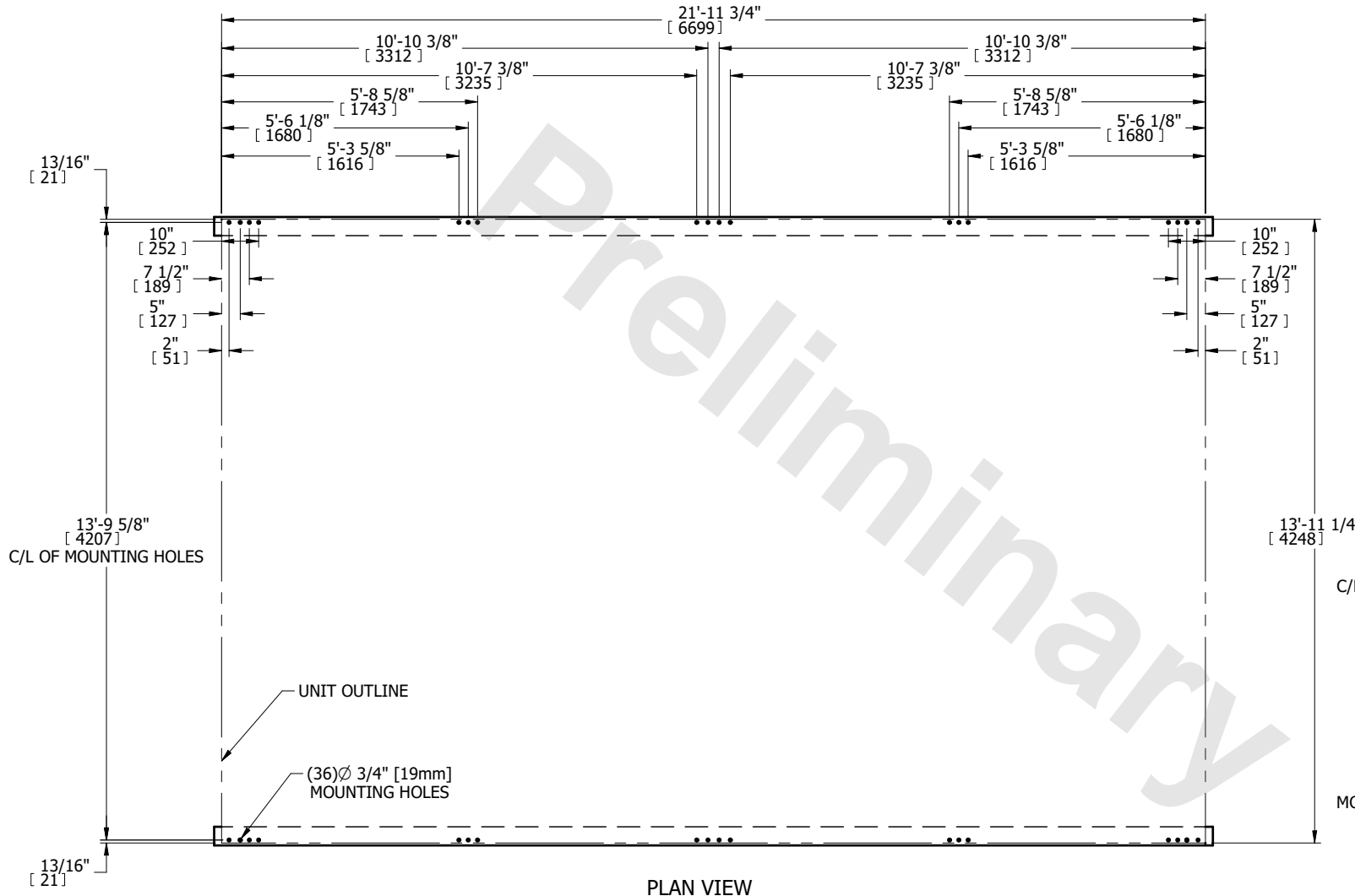
PLAN VIEW
