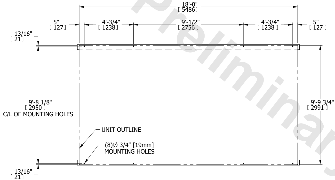
PLAN VIEW
