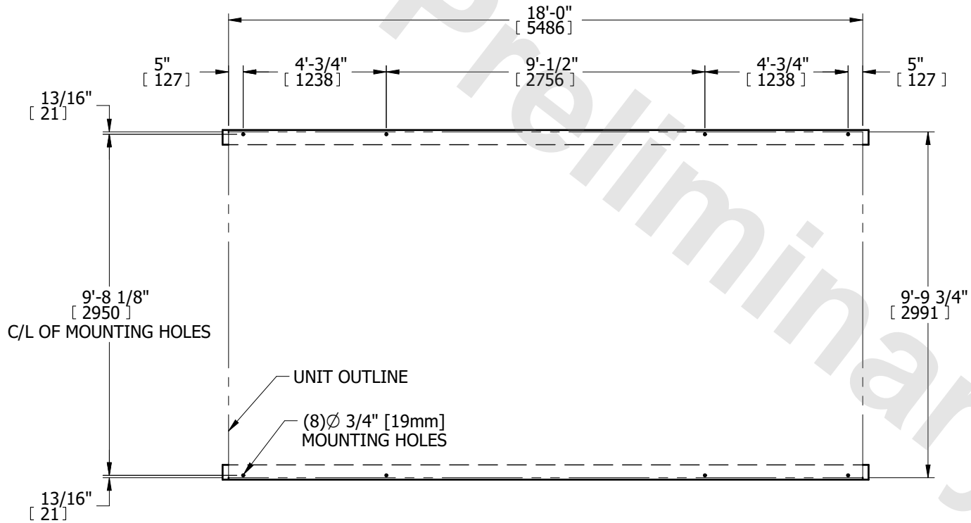
PLAN VIEW
