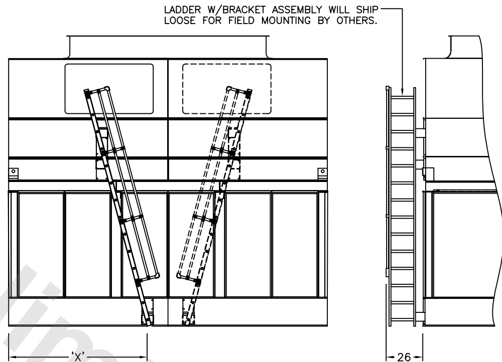
SIDE VIEW
