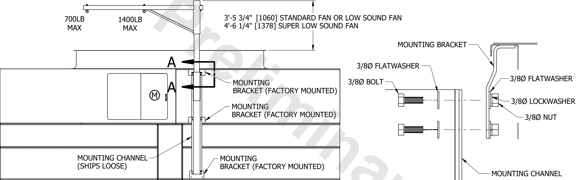
SECTION A-A ASSEMBLY ARRANGEMENT (TYPICAL)
