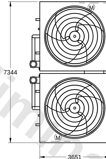
PLAN VIEW
