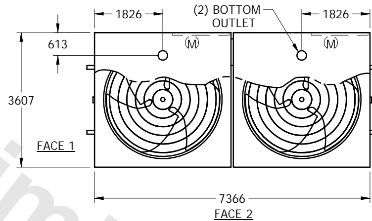
PLAN VIEW
