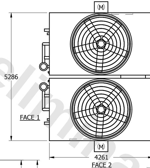
PLAN VIEW
