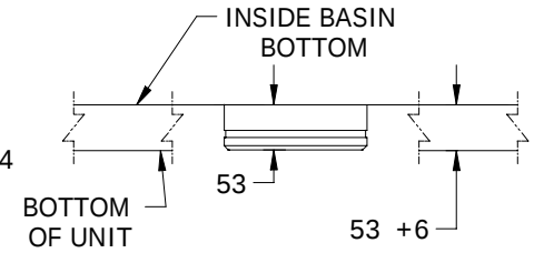
TYPICAL BOTTOM INLET CONNECTION DETAIL
