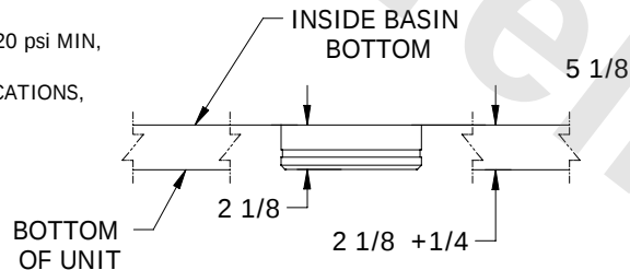
TYPICAL BOTTOM INLET CONNECTION DETAIL
