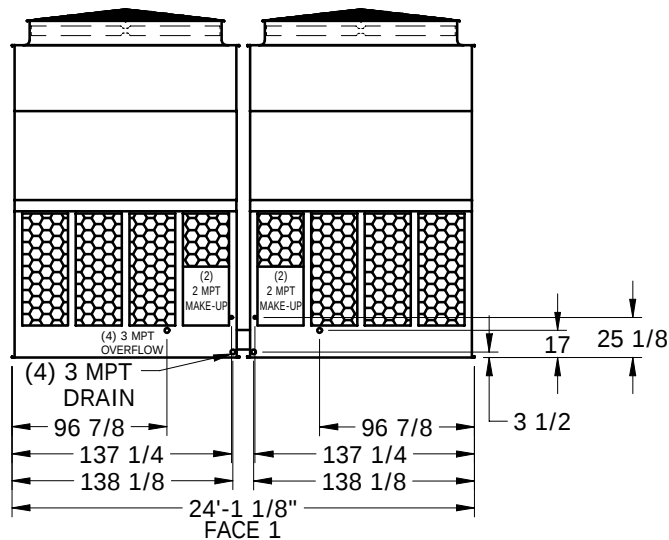
TYPICAL BOTTOM INLET CONNECTION DETAIL
