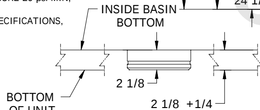
TYPICAL BOTTOM INLET CONNECTION DETAIL
