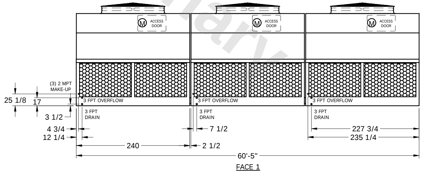
TYPICAL BOTTOM INLET CONNECTION DETAIL
