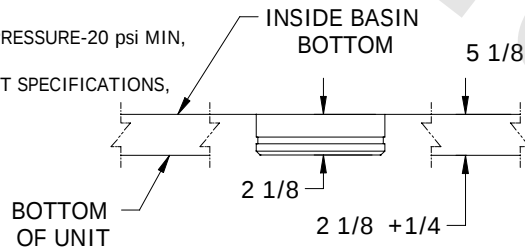
TYPICAL BOTTOM INLET CONNECTION DETAIL
