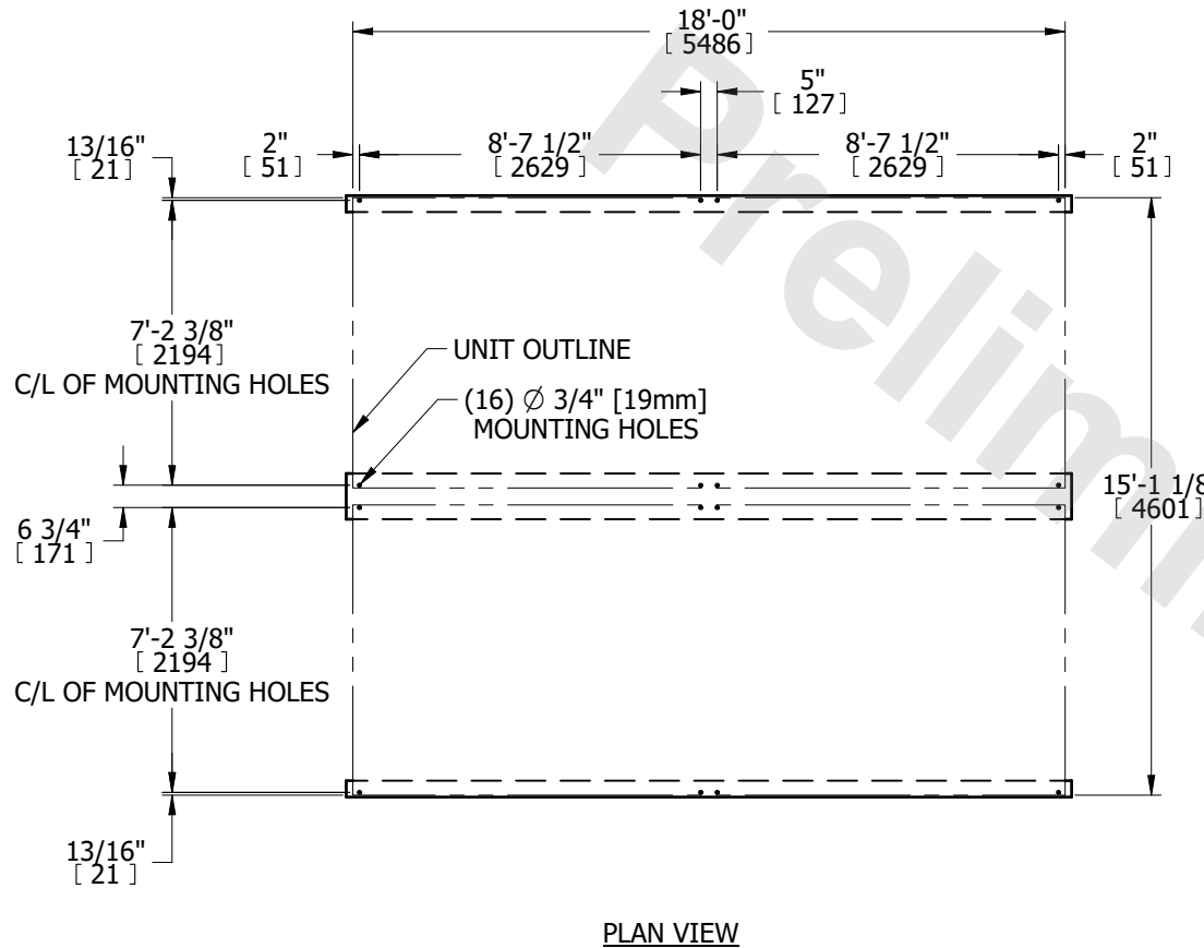
PLAN VIEW
