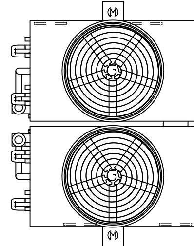
FACE 2 PLAN VIEW
