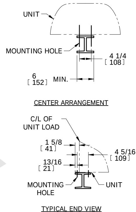
TYPICAL END VIEW
