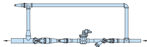
Single Liquid Feed Assembly (LFA) with Hand Expansion Valve (HX)
