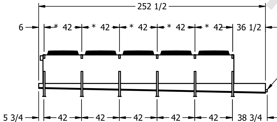
2" MPT DRAIN
