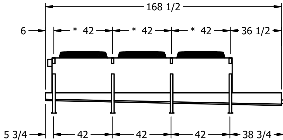
2" MPT DRAIN
