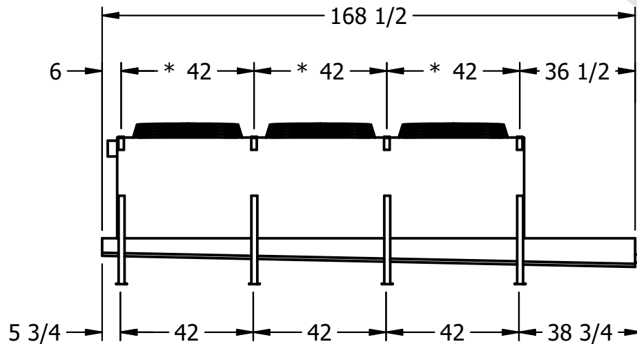
2" MPT DRAIN
