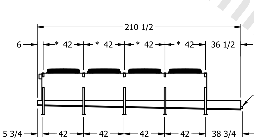
2" MPT DRAIN
