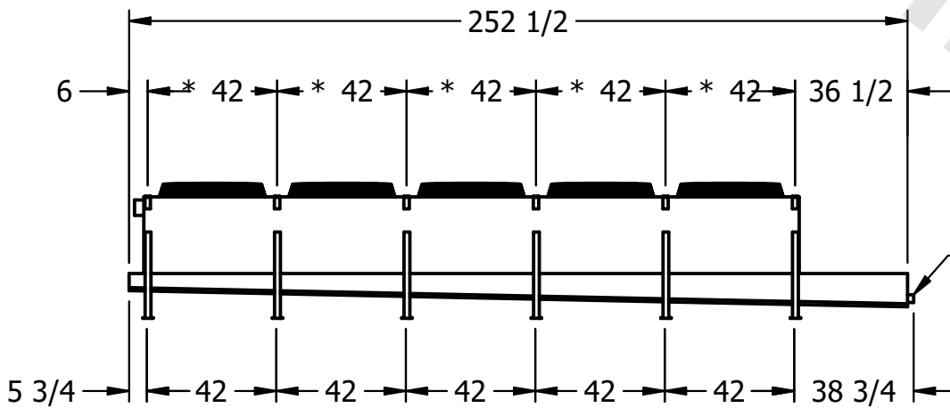
2" MPT DRAIN
