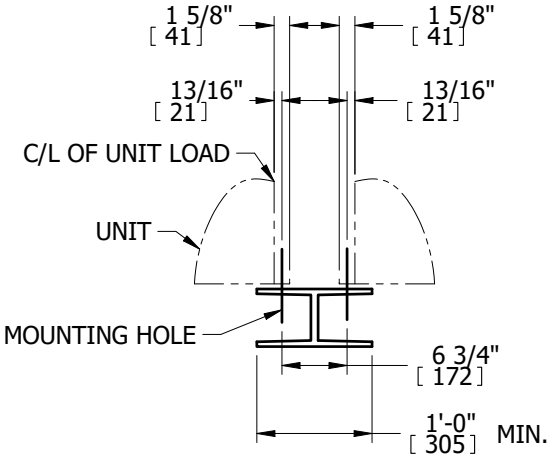
CENTER ARRANGEMENT
