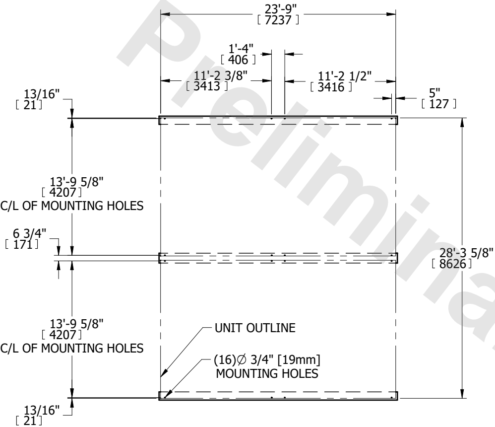
PLAN VIEW
