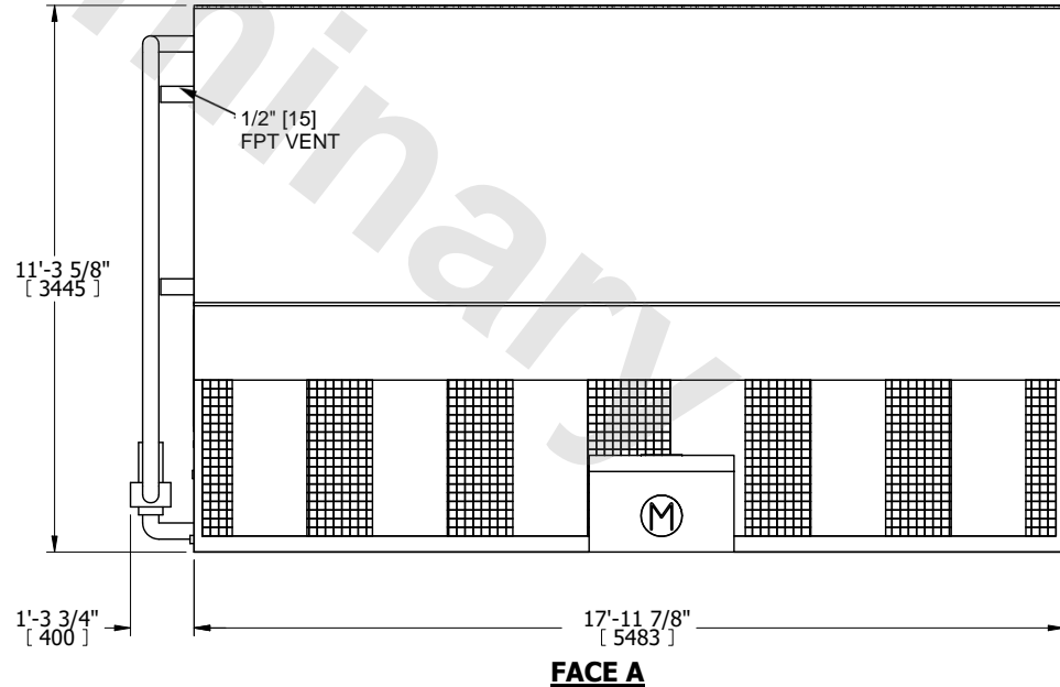
FACE A
