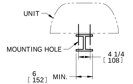
CENTER ARRANGEMENT
