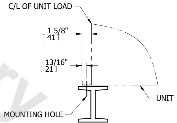
TYPICAL END VIEW
