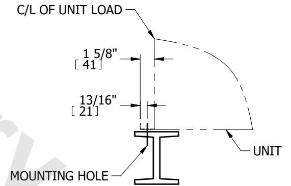
TYPICAL END VIEW
