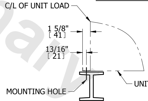
CENTER ARRANGEMENT
