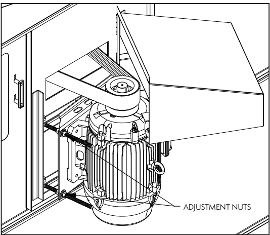
Figure 3 — Externally Mounted Motors, AT Units
