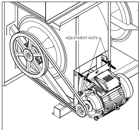
Figure 4 — Externally Mounted Motors, 4' and 5' LSTE Units
