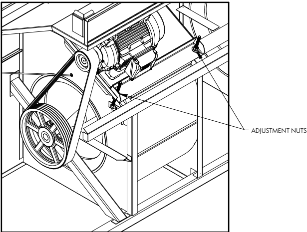
Figure 5 — Externally Mounted Motors, 8' and 10' LSTE Units
