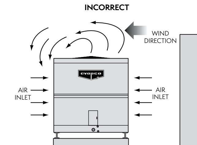
Figure 24 — Wind Effect with Top of Unit Lower than Top of Wall
