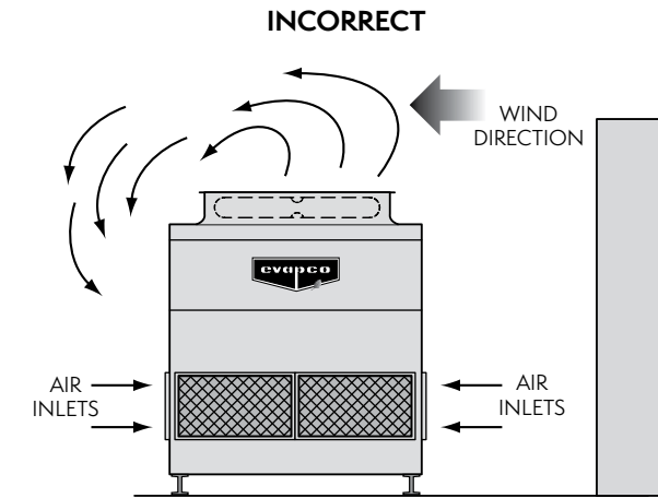
Figure 2 — Wind Effect with Top of Unit Lower than Top of Wall
