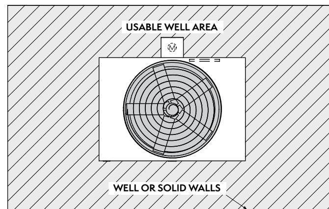
Figure 20 — Well Installation
