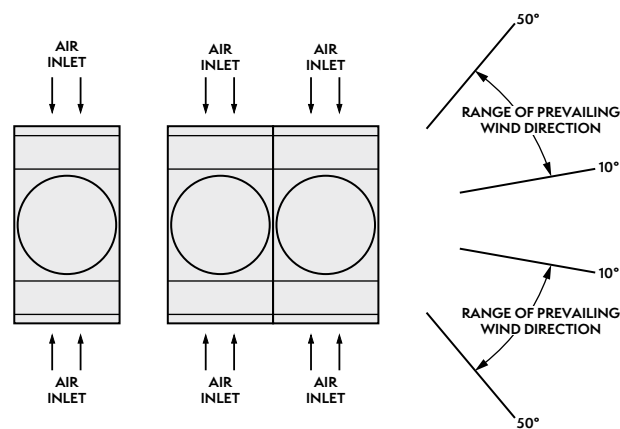
Figure 29 — Prevailing Wind
