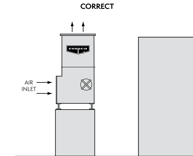
Figure 35 — Installation Elevated so Top of Unit is Higher than Top of Wall
