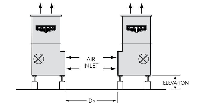
Figure 43 — Installation with Air Inlets Facing Each Other
