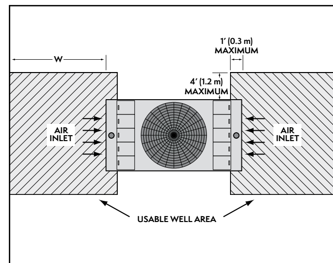
Figure 30 — Well Installation
