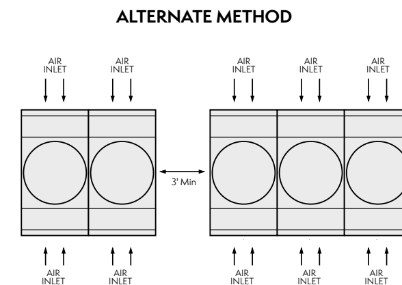
Figure 28a — Multiple Units Placed End-to-End
