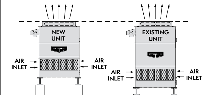
Figure 22 — Expansion to an Existing Installation
