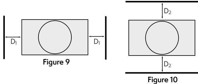
CASE 4 – Two Walls/Two Units
