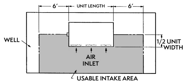
Figure 46 — Well Installation
