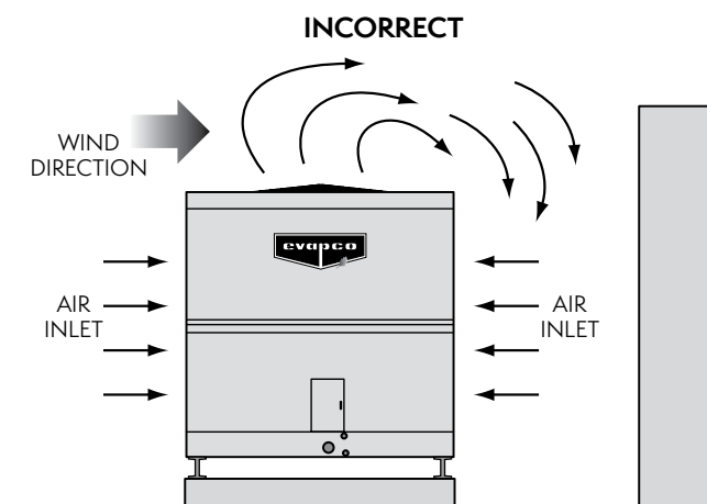
Figure 23 — Installation with Top of Unit Lower than Top of Wall
