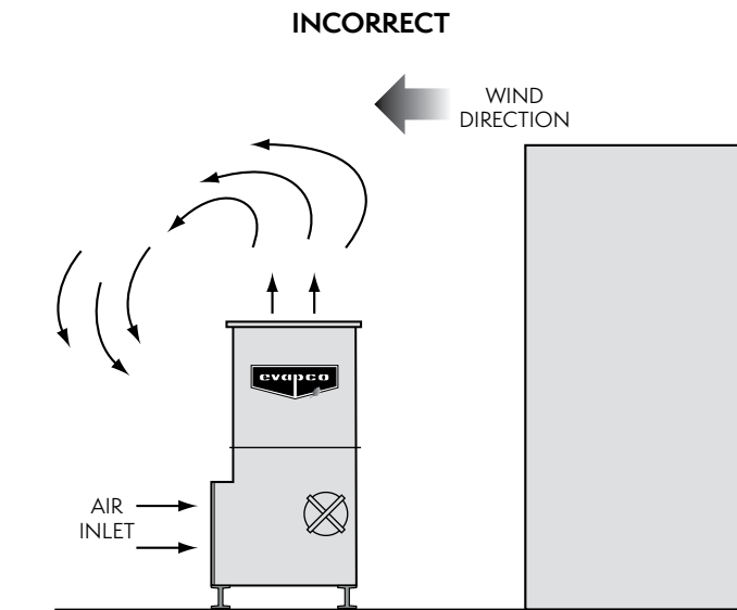
Figure 34 — Wind Effect with Top of Unit Lower than Top of Wall
