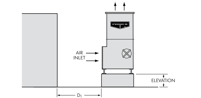
Figure 38 — Installation Next to Wall
