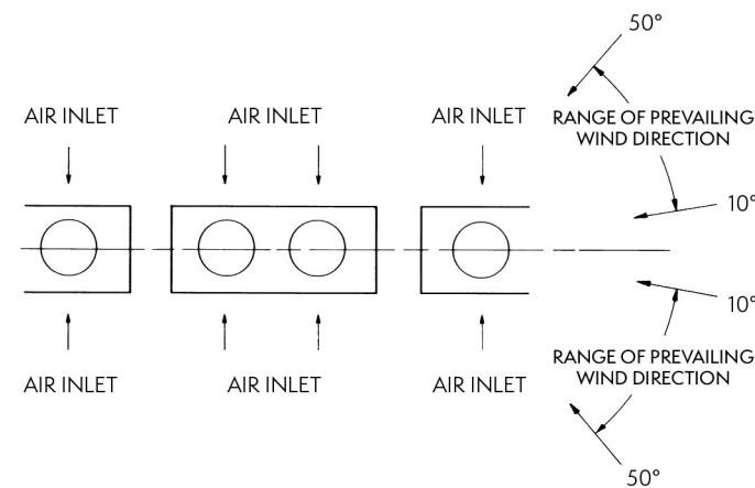
Figure 19 — Prevailing Wind
