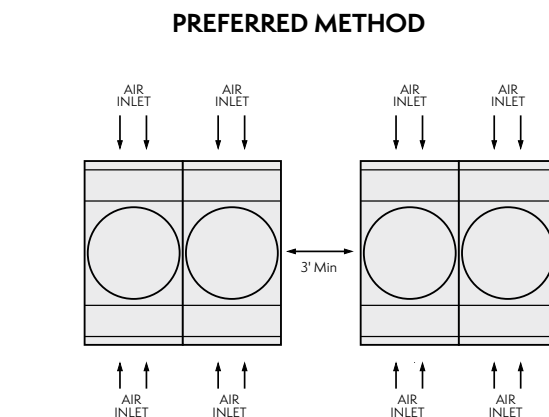
Figure 28 — Multiple Units Placed End-to-End
