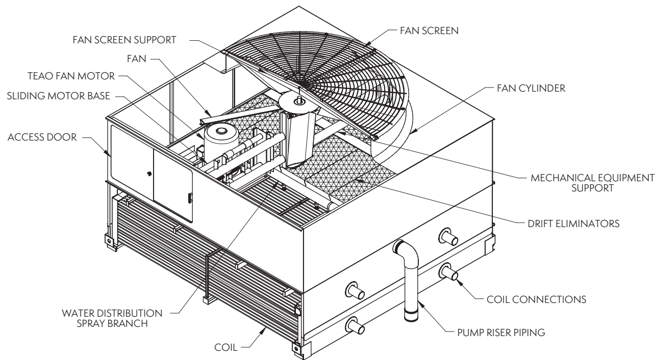
FAN & COIL CASING SECTION
