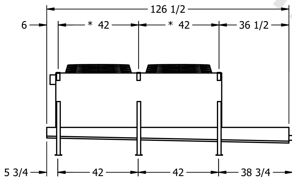
- 2" MPT DRAIN
