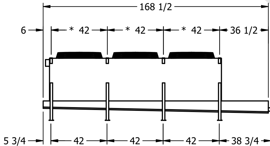
2" MPT DRAIN
