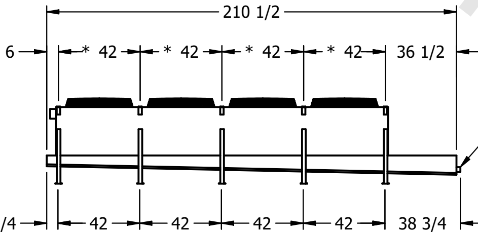
2" MPT DRAIN
