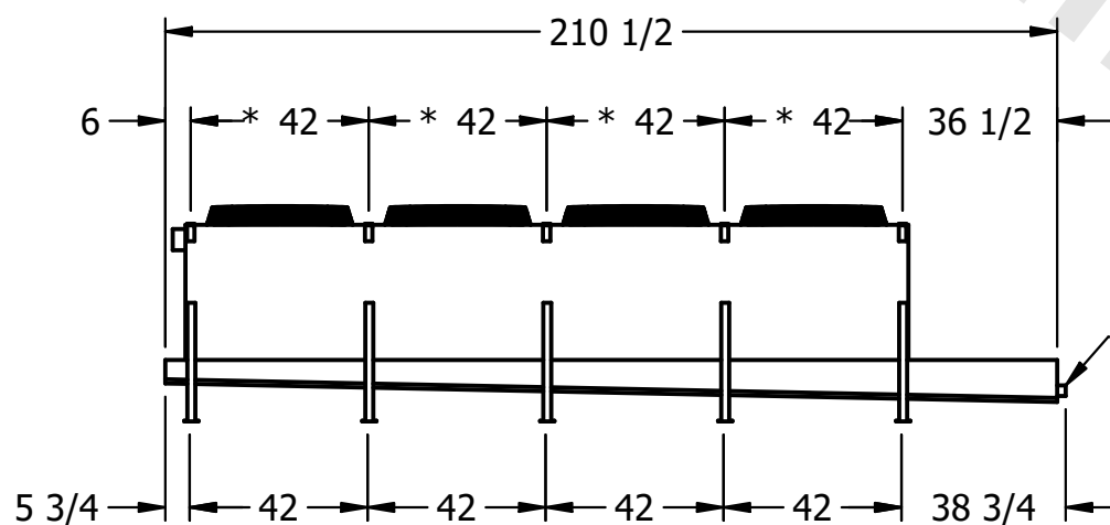
- 2" MPT DRAIN
