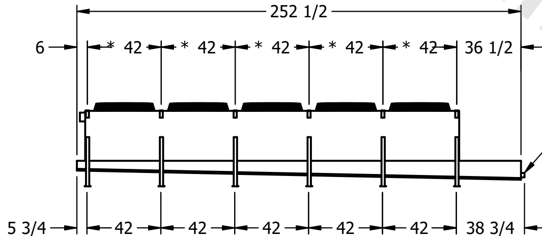
2" MPT DRAIN
