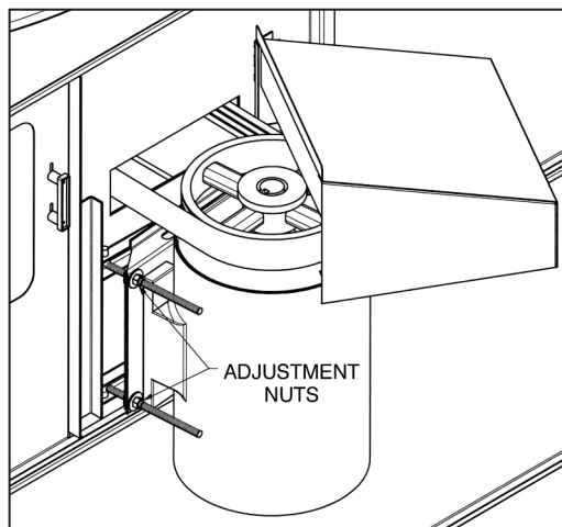
Figure 3 – Externally Mounted Motors, AT/UT/USS Units
