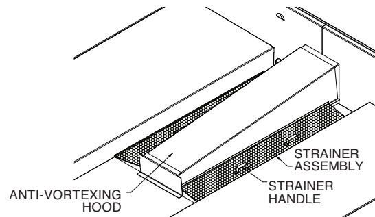
Figure 12 – AXS Strainer Assembly
