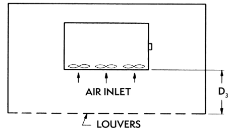
Figure 47 — Louvered Wall Enclosure with Front Louvers
