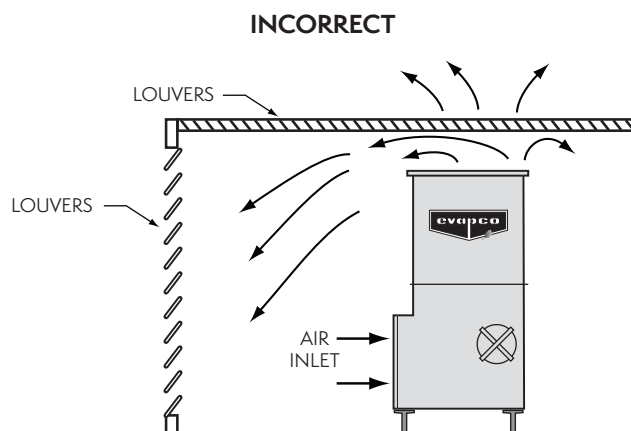
Figure 48 — Louvered Enclosure with Grating Over Top
