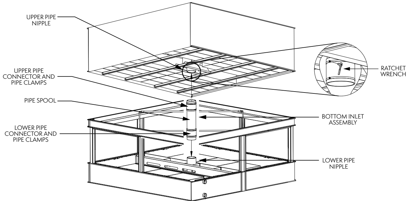
Figure 29 – Bottom Inlet Riser Pipe Installation
