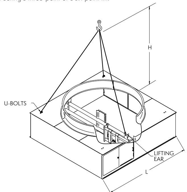
Figure 8 – Three-Point Lift
