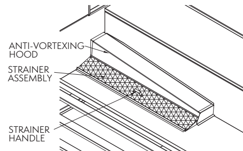
Figure 13 — PHC-S/PHC-L Strainer Assembly
