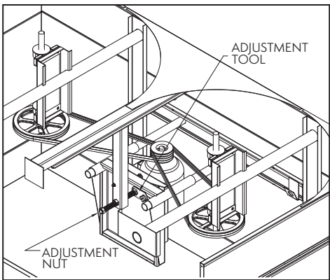
Figure 6 — Internally Mounted Motor, PHC-S & L Tandem Fan Units
