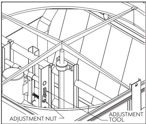
Figure 5 — Internally Mounted Motor, PHC-D Unit
