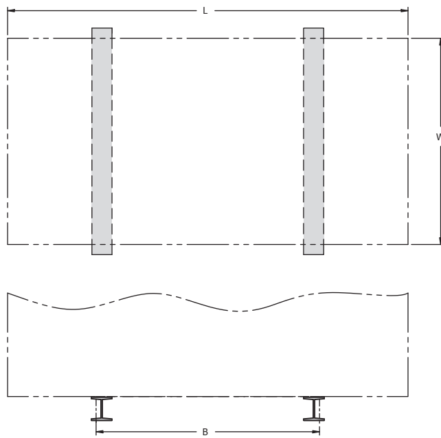
Transverse Steel Support Arrangement
