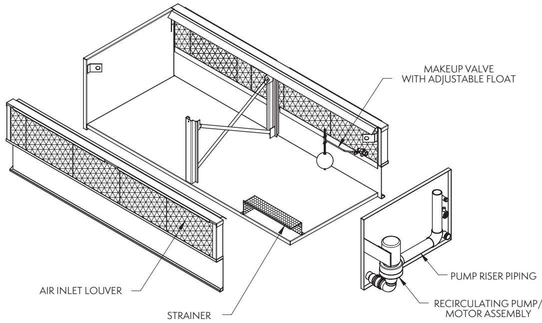
PAN SECTION
