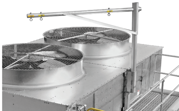
ATC-E Condenser with Optional Service Platform and Motor Davit
