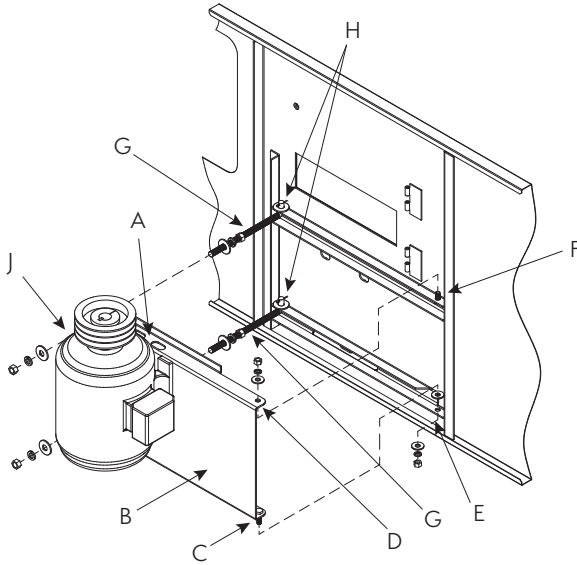
Figure 17a – External Motor Installation
