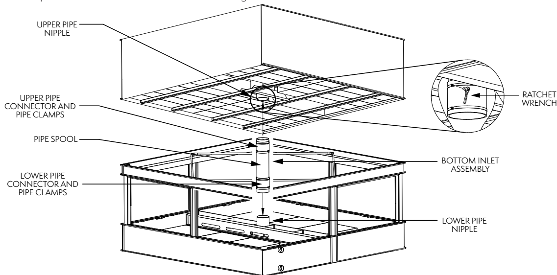
Figure 30 – Bottom Inlet Riser Pipe Installation
