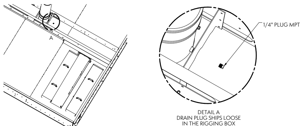
Figure 31 – Weep Hole
